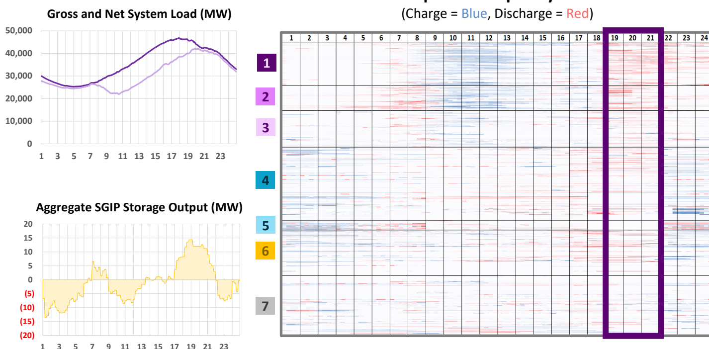
Figure 17: Nonresidential SGIP storage project performance during CAISO stage 3 emergency on August 14, 2020
