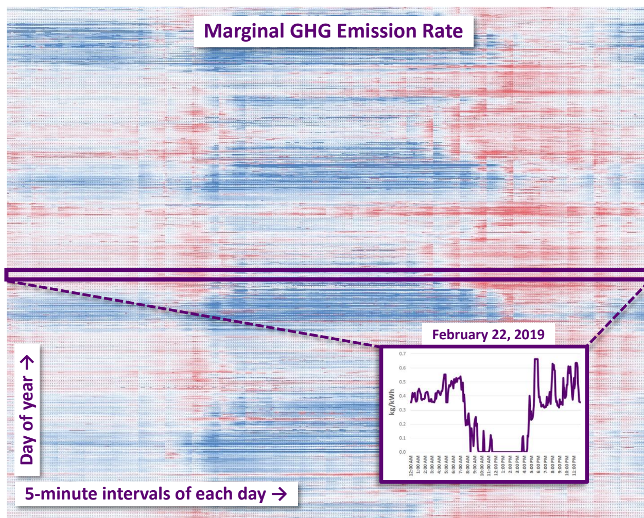
Figure 22: Heatplot of historical marginal GHG emission rates used in the study
