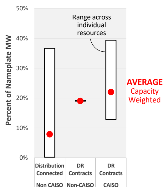
Figure 19: Observed capacity contribution of distribution- and customer-sited storage
